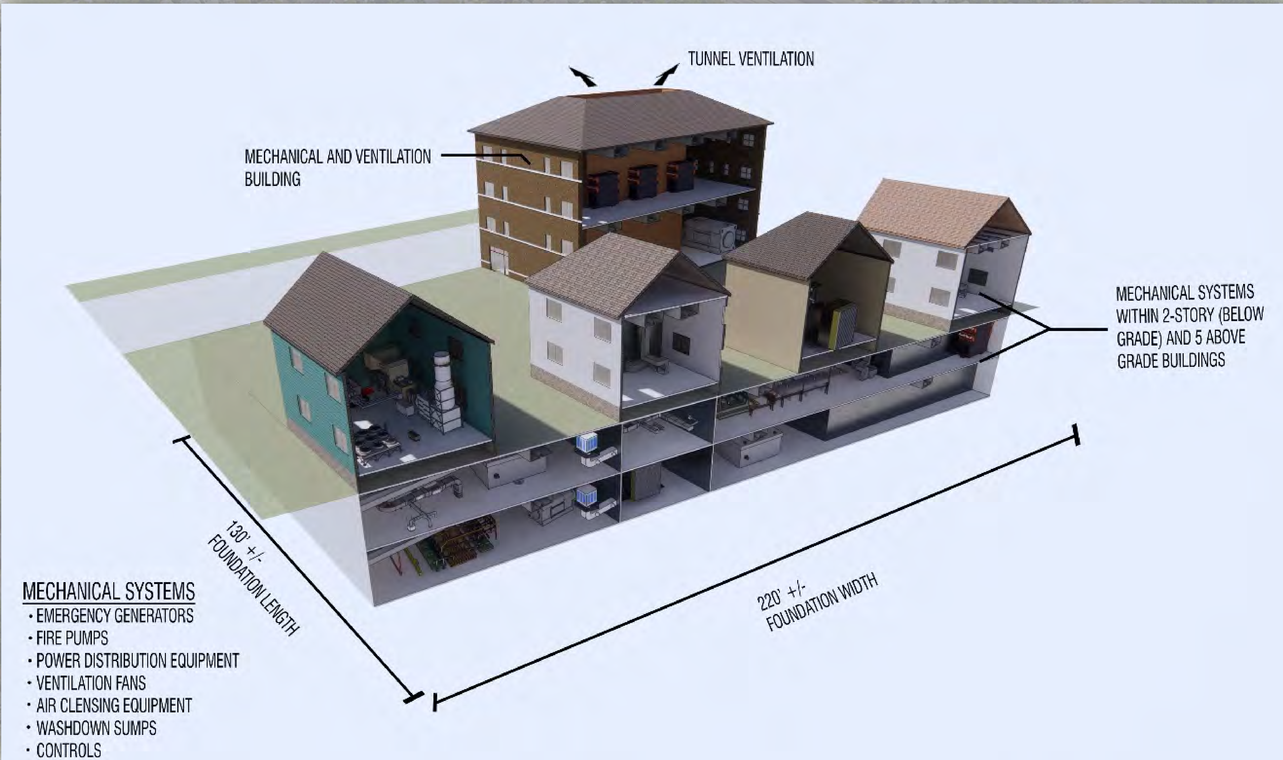
Single (130' by 220') Utility Building Complex
